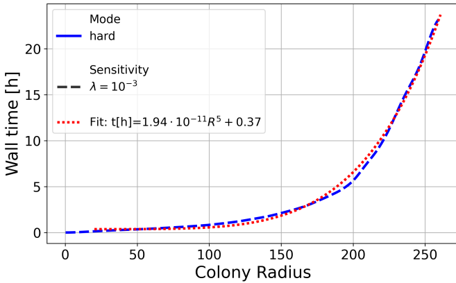
Figure 18: Wall time as a function of colony radius. The wall time roughly follows T_{\text{wall}} [\text{h}] \approx 1.94 \cdot 10^{-11} R^5 + 0.37 .
