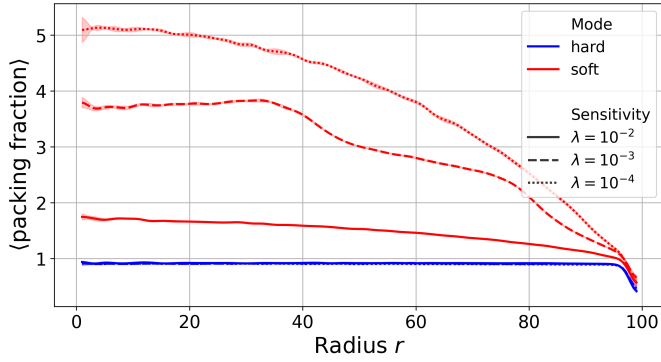
(a) Radial packing fraction profiles ( \phi = \frac{A_{\text{cells}}}{A_{\text{total}}} ) for both models. Here A_{\text{cells}} is the total area occupied by cells within a radial bin of width 2 at distance r from the colony center, and A_{\text{total}} is the annular area of that bin. The hard model maintains nearly optimal packing, while the soft model exhibits higher fractions in the colony center, especially at low stress-sensitivity ( \lambda = 10^{-4} ).
