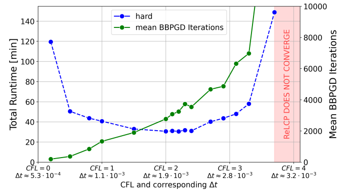
Figure 16: Total runtime to reach a colony radius of 100 versus CFL number on 112 cores. The red region indicates CFL values where the ReLCP procedure fails to converge.
