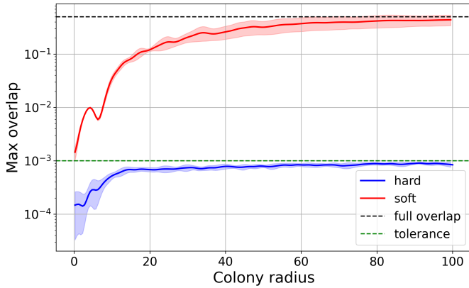
(b) Maximum cell overlap over simulation time. The hard model maintains overlap near the solver tolerance \epsilon = 10^{-3} , while the soft model exhibits a steady increase, reaching near-complete overlap by the simulation end.
