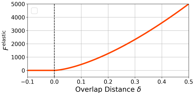
Figure 3: Hertzian contact model. When two spherocylindrical cells overlap by a distance \delta , they experience a repulsive elastic force \mathbf{F}^{\text{elastic}} . The force acts along the normal vector \hat{\mathbf{n}} at the contact point.
