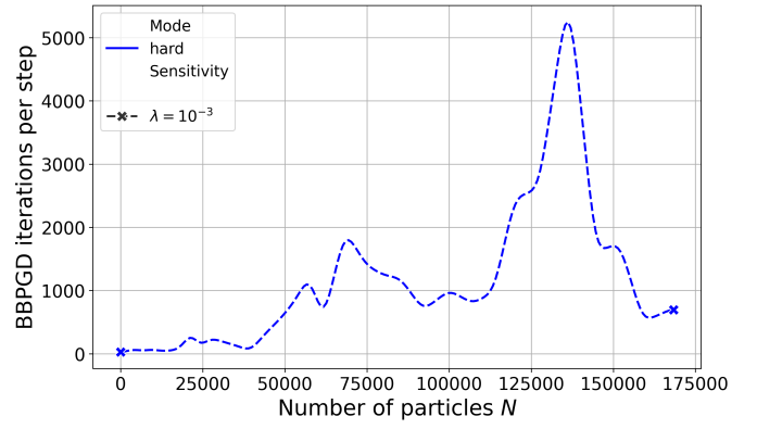
(a) Number of BBPGD iterations per timestep as a function of particle count. Iterations remain roughly \mathcal{O}(1000) on average, with occasional spikes up to \mathcal{O}(5000) .
