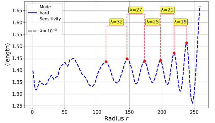
(b) Radial distribution of the average cell length for the hard model at R = 260 . The oscillatory pattern has a characteristic wavelength of \lambda \approx 25 , corresponding to the radial ring spacing visible in Figure A1.
