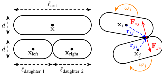
Figure 2: Spherocylinder cell model. Contact forces \mathbf{F}_{ij} (red) and lever arms \mathbf{r}_{ij} (dashed blue) generate torques causing angular motion \boldsymbol{\omega} (orange), and also produce translational displacements of the cells. Cell division occurs when a cell reaches critical length \ell_{\text{crit}} .
