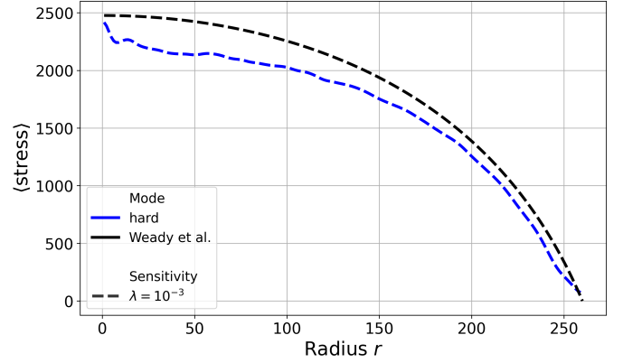
(c) Radial stress profile of the hard model at R = 260 . The simulated stress closely follows the analytical prediction from [23], confirming global mechanical balance across the colony.
