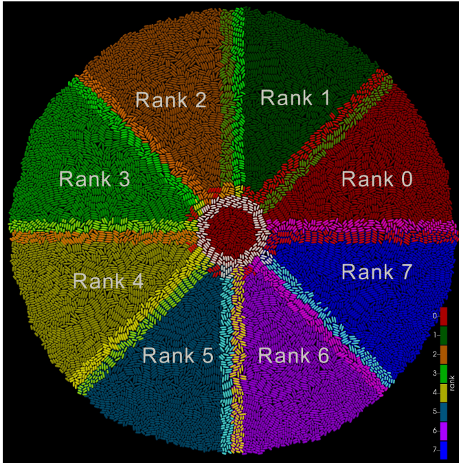
Figure 13: Domain decomposition for 8 MPI ranks showing evenly spaced angular sectors of a colony with radius 50. Each rank owns one angular sector. Ghost particles at rank boundaries are shown in brighter colors.
