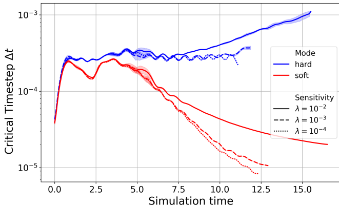
Figure 15: Adaptive timestep \Delta t for both collision models. The soft model requires a drastic reduction of \Delta t ( \Delta t_{\text{soft}} \approx 10^{-5} ) to maintain stability, whereas the hard model maintains a significantly larger timestep ( \Delta t_{\text{hard}} \approx 3 \cdot 10^{-4} ), allowing more computation per communication step.
