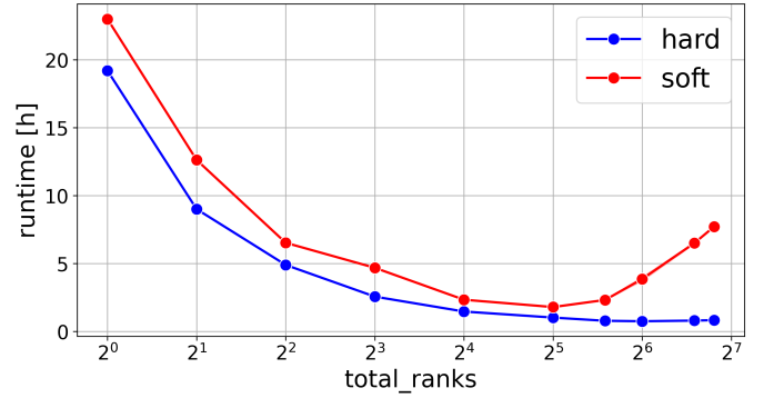
(a) Runtime to reach colony radius of 100 versus CPU cores. The hard model is consistently faster, with the performance gap widening at high core counts.
