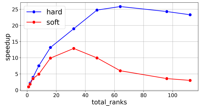
(b) Speedup versus CPU cores. The hard and soft models scale reasonably up to 64 and 32 cores, respectively.
